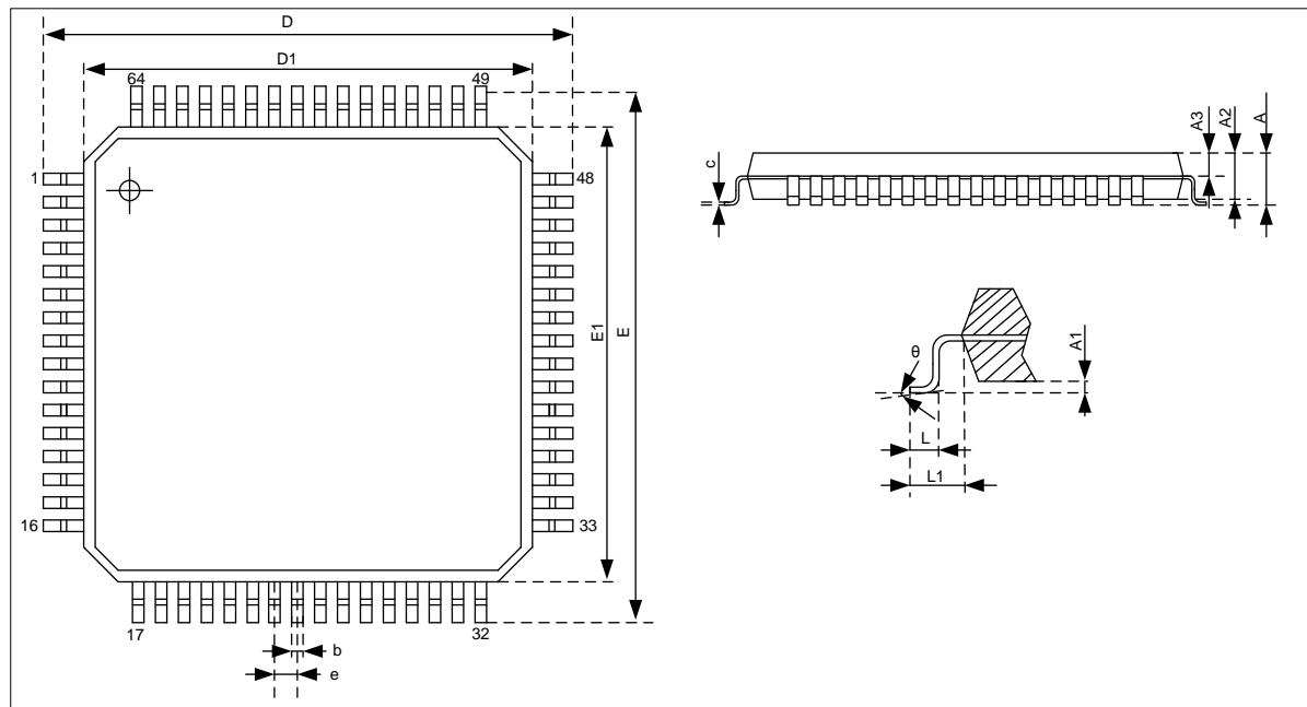
LQFP64
