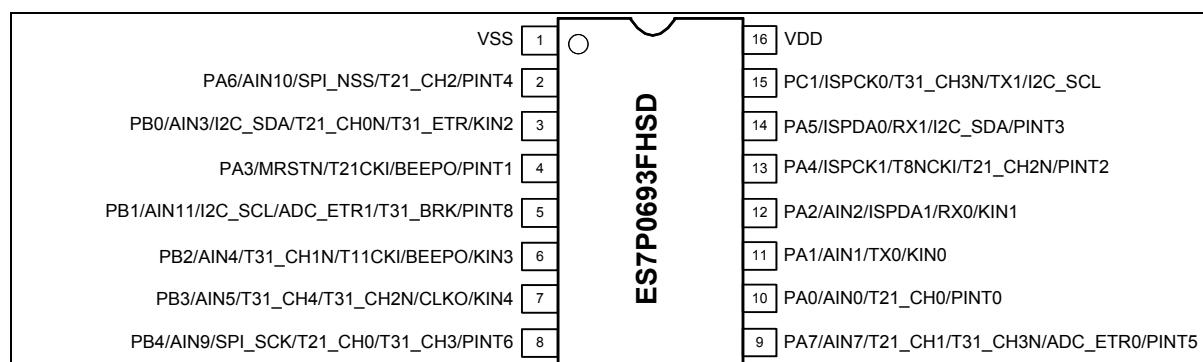
1.4.3 16-pin (SOP)
