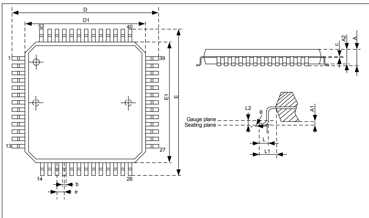
LQFP52
